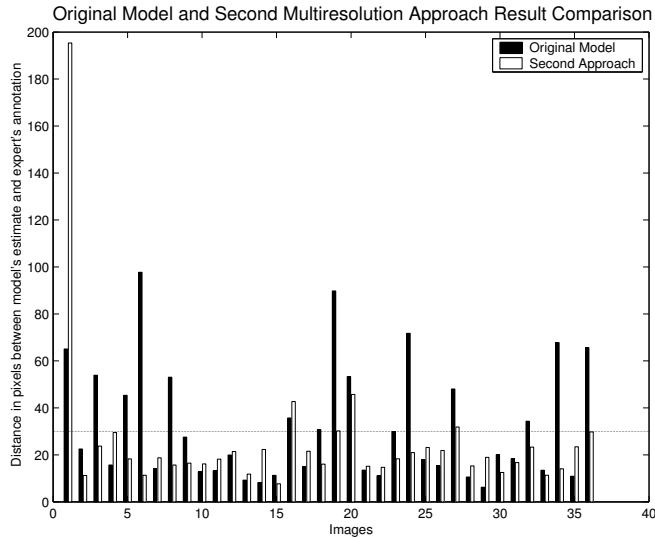
Fig. 4. Comparison of original model and second multiresolution approach test results.
